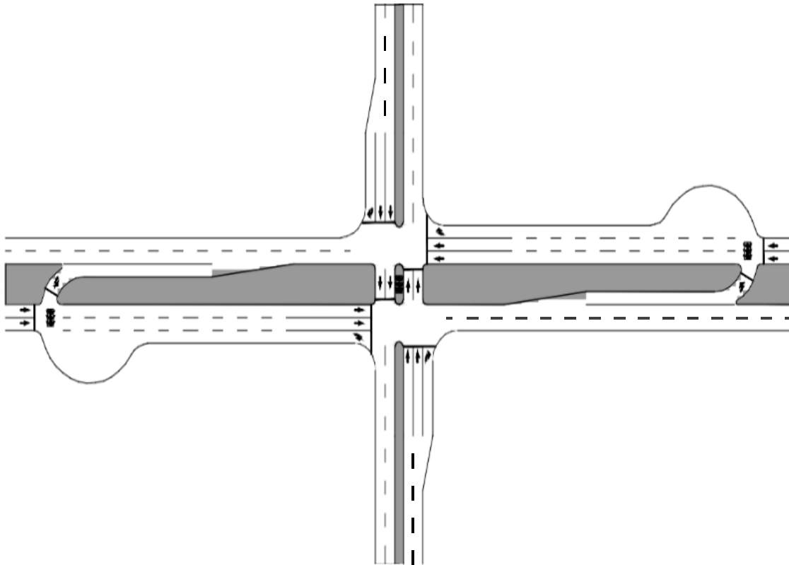
MUT Intersection from FHWA's Median U-Turn Intersection Informational Guide
