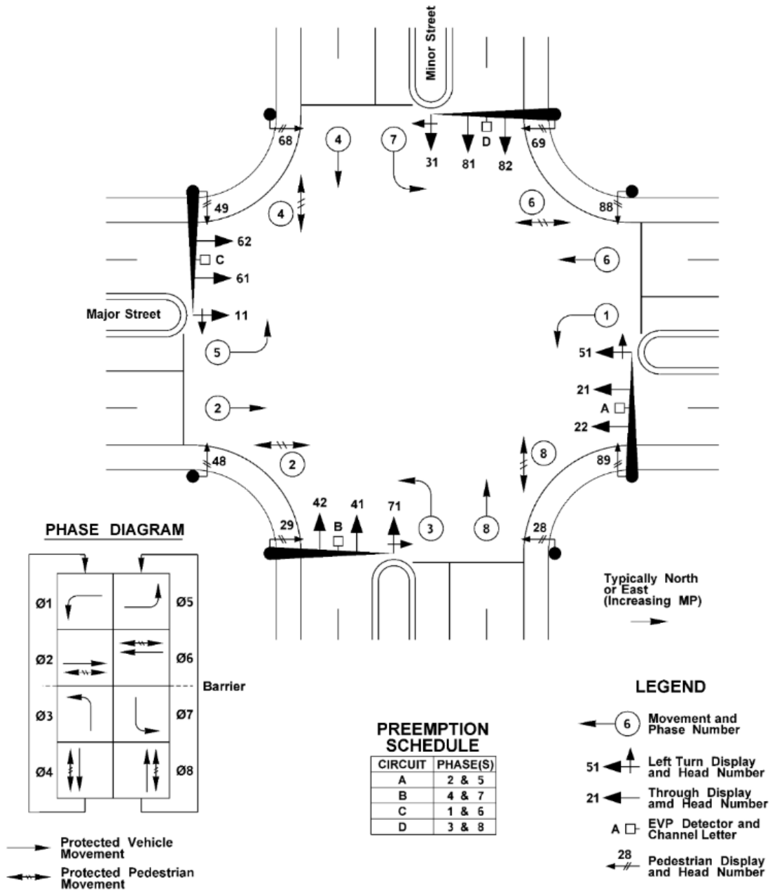
Exhibit 1330-5 Standard Intersection Movements, Head Numbers, and Phase Operation
