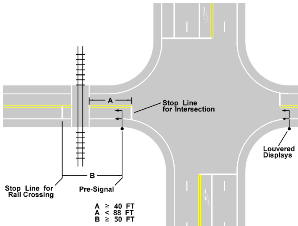
Display Placement – 40 to 88 feet between tracks and intersection
