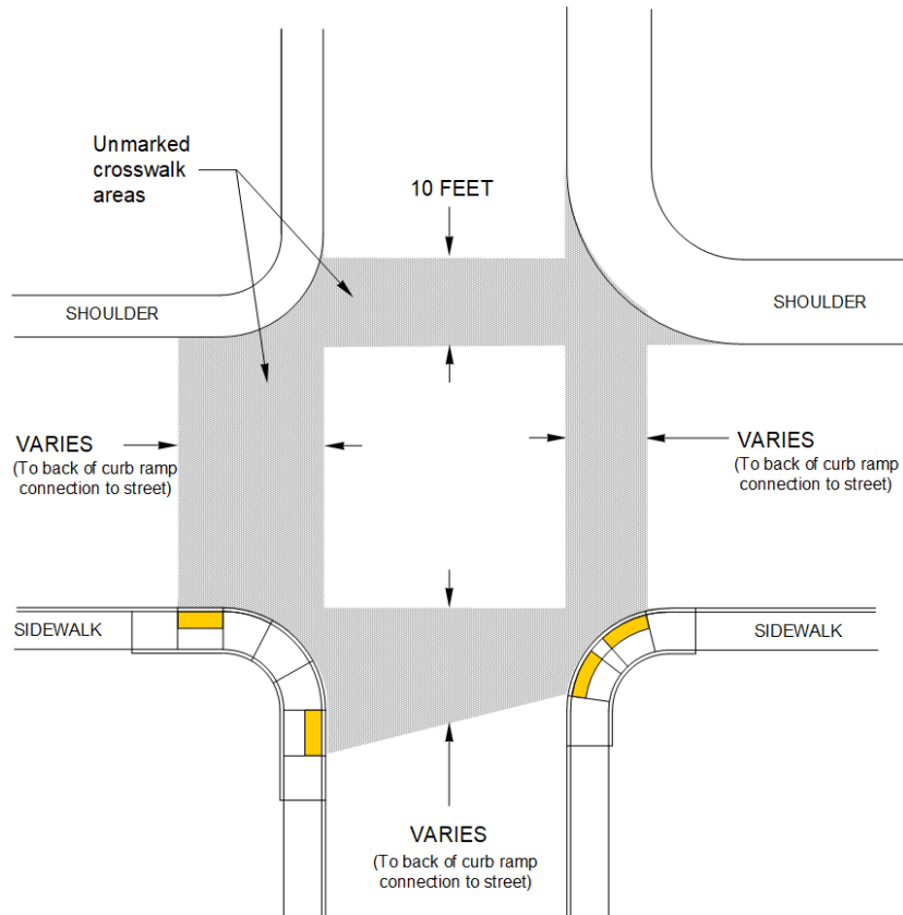
Exhibit 1510-21 Unmarked Crosswalks
