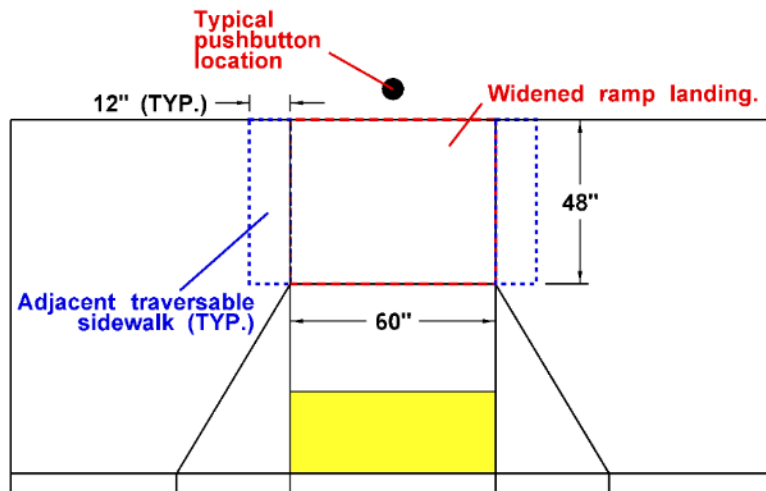
Perpendicular Ramp Option: Widen Ramp and Landing (Not to scale)
