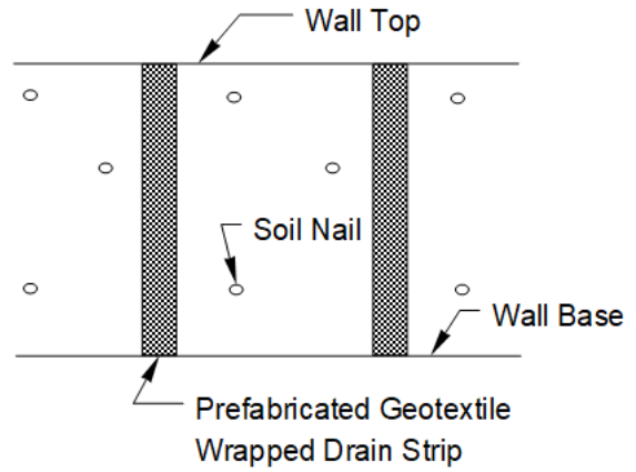
O. Prefabricated Drain Strip Behind Wall Face
