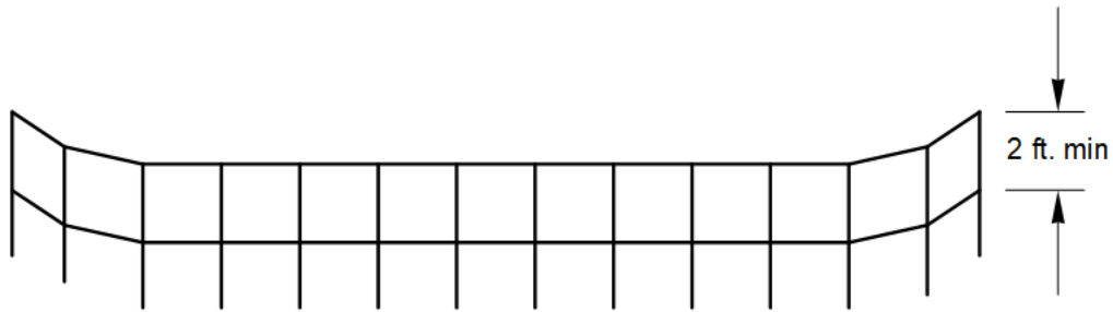
Silt Fence Profile
