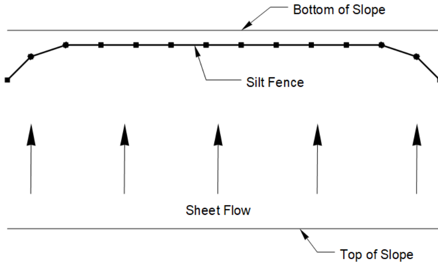
Silt Fence Plan
