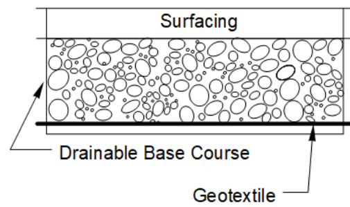
D. Underground Drainage: Moderate Survivability (Area Drain Under Parking Lot or Roadway)
