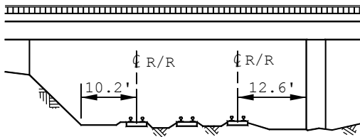
RAILROAD MULTIPLE TRACK EXAMPLE
