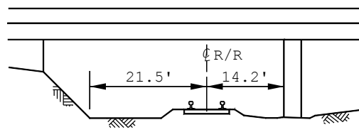
RAILROAD SINGLE TRACK EXAMPLE
