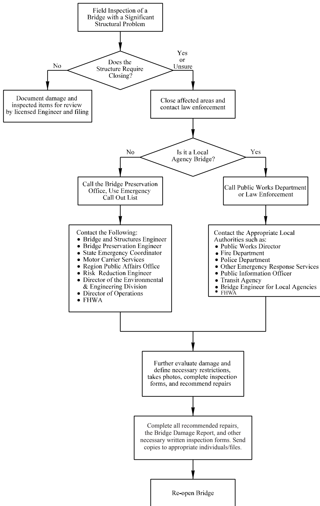
Field Inspection Procedure Figure 6.02-A
