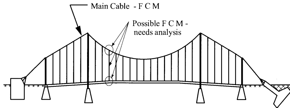
Example A: Cable Suspension Bridge
