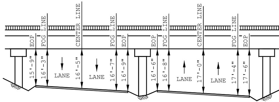
DIVIDED HIGHWAY EXAMPLE
