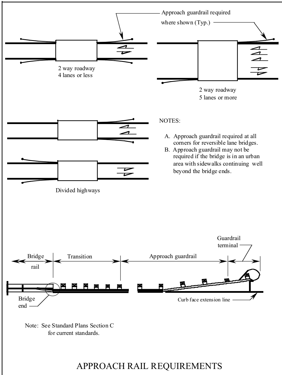
Approach Rail Requirements Figures WB76-84 through WB76-87
