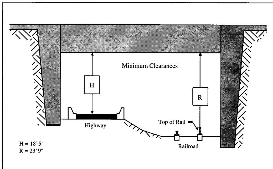
Vertical Clearances Figure WB73-78
