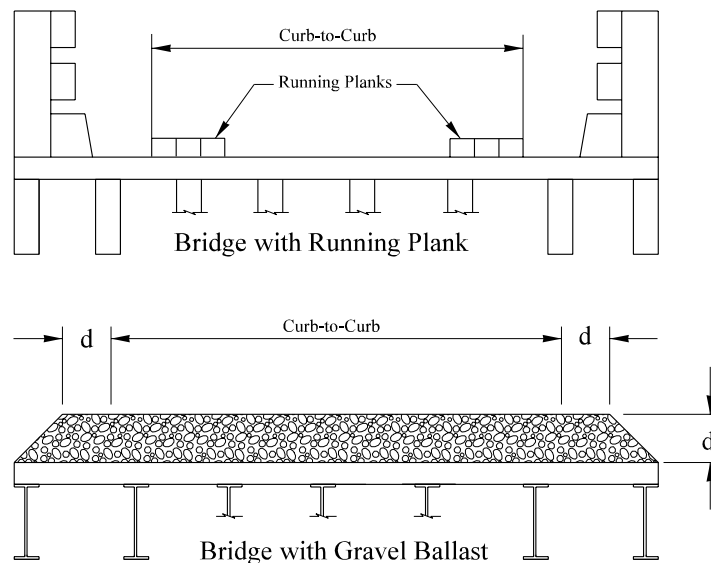
Curb-to-Curb Roadway Width Figure WB73-56
