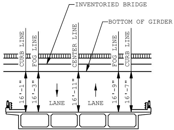
BRIDGE OVER BRIDGE EXAMPLE
