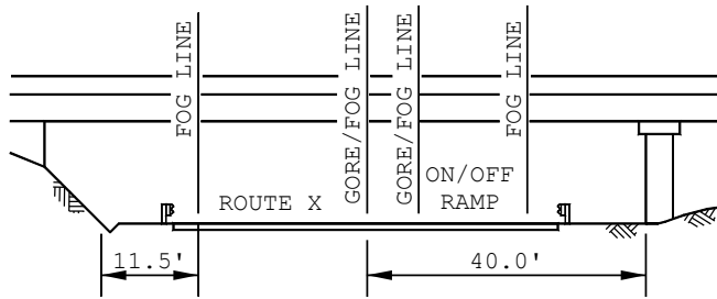
HIGHWAY ON/OFF RAMP EXAMPLE
