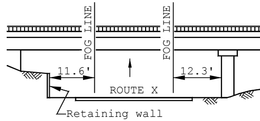
HIGHWAY WITH RETAINING WALL EXAMPLE
