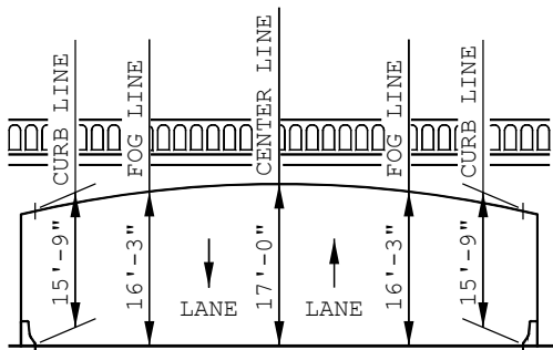
UNDIVIDED HIGHWAY EXAMPLE
