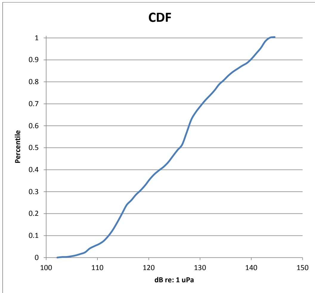
Figure 7: Cumulative Distribution Function (CDF) plot for the broadband hourly RMS background noise level data.
