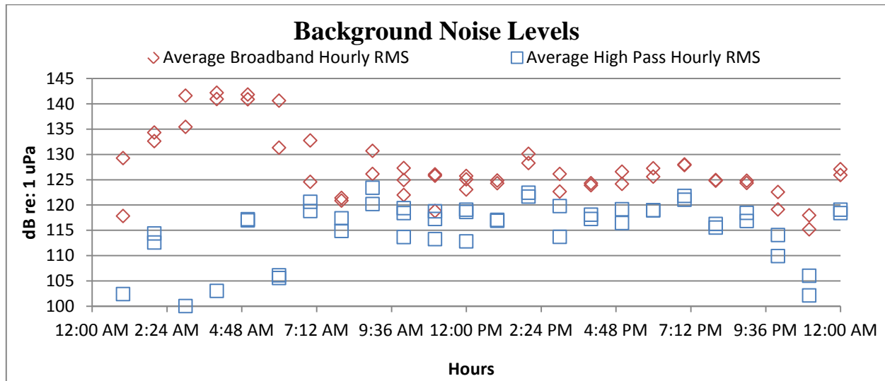
Figure 5: Hourly average RMS values with and without the high pass filter applied.
