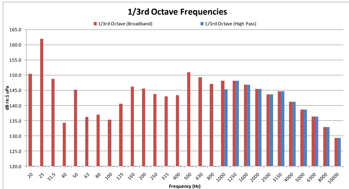
Figure 2: 1/3 rd octave analysis of the broadband versus the high pass filtered data.
