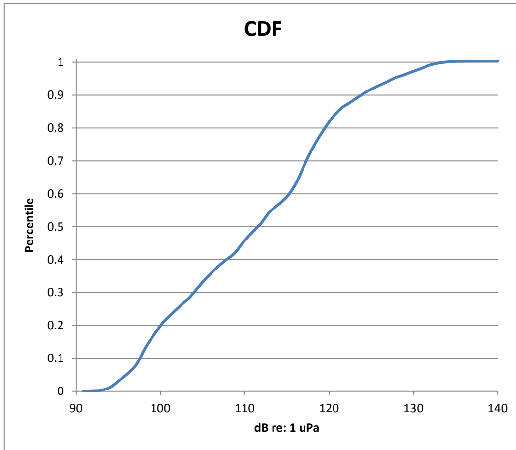
Figure 8: Cumulative Distribution Function (CDF) plot for the high pass filtered hourly RMS background noise level data.
