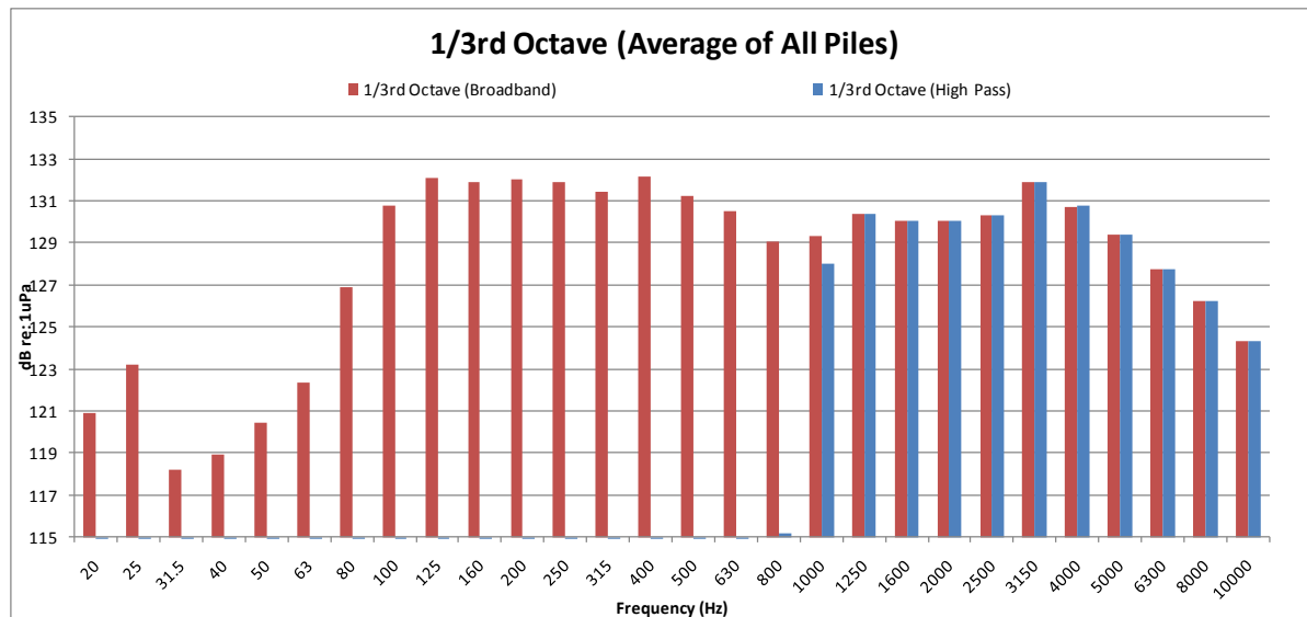
Figure 3: 1/3 rd octave analysis of the broadband versus the high pass filtered data averaged for all 6 piles.
