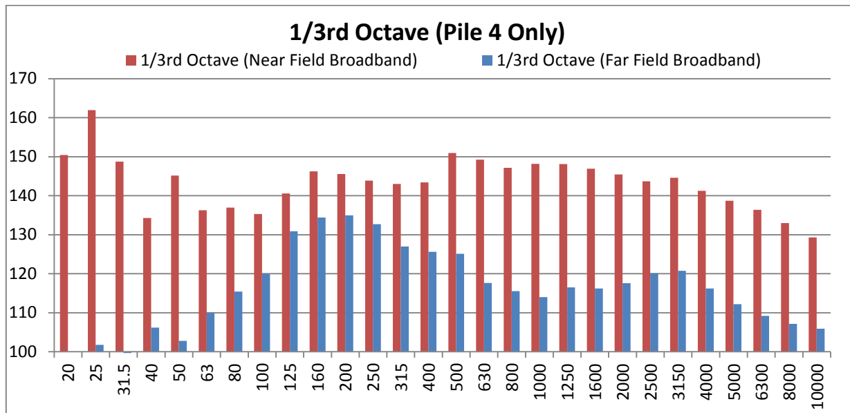
Figure 4: 1/3 rd octave analysis of the broadband near field versus far field data for Pile 4 only.
