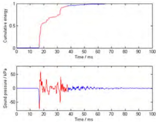
Figure A1. Illustrating the definition of the time span corresponding to 90 percent of the energy of a broadband pulse. The time span, the red segment in lower left panel, was determined by squaring and integrating the pulse in a cumulative sense (upper left panel), after which the 0.05-to-0.95 energy time duration was determined. SEL was then computed over this time duration, as shown in the right panel, and this same time duration was used to compute the RMS pressure.
