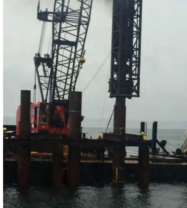
Figure 3b. The three piles in the template, taken on 8 December. The control pile is on the left, the double wall pile is in the middle, and the mandrel pile is on the right.
