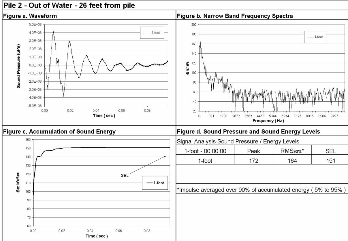
Figure 7: Waveform Analysis of Pile 2 Underwater Sound Pressure Levels 26-feet from the pile driven outside the water channel.
