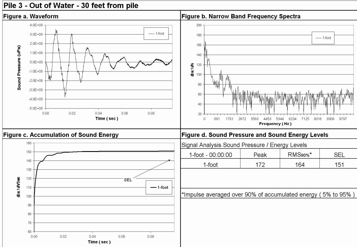
Figure 8: Waveform Analysis of Pile 3 Underwater Sound Pressure Levels 30-feet from the pile driven outside the water channel.
