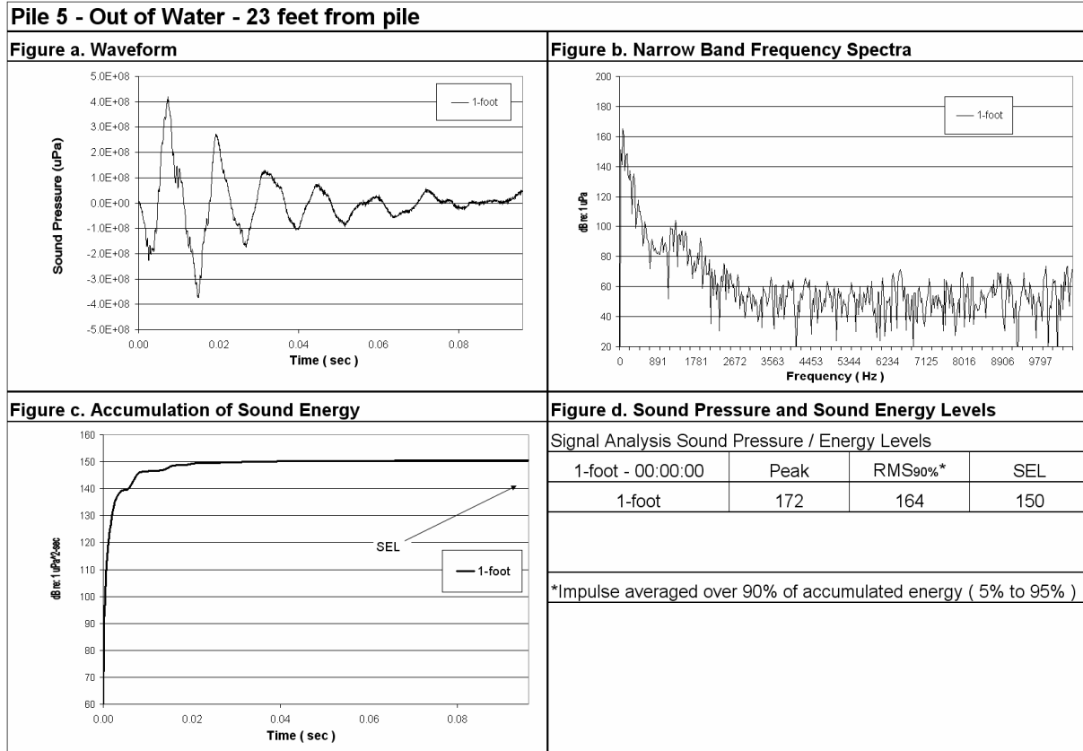
Figure 10: Waveform Analysis of Pile 5 Underwater Sound Pressure Levels 23-feet from the pile driven outside the water channel.
